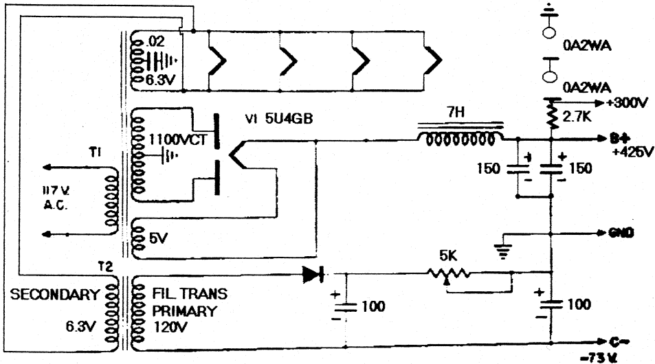
TRIOPHONI POWER SUPPLY SCHEMATIC MODIFIED FROM ELECTRONICS WORLD, JULY, 1958, P. 62
